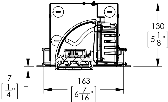
SECTION H-H SCALE 1 : 4
