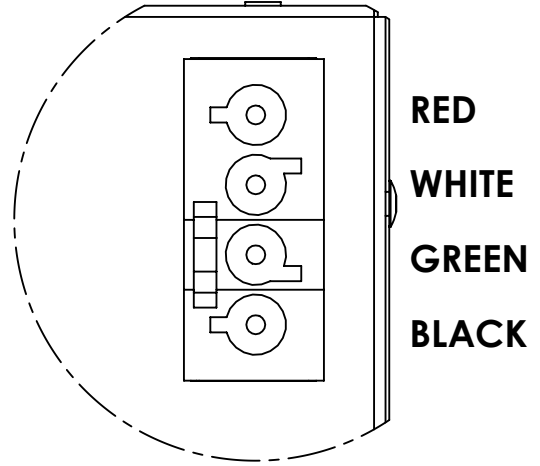
DETAIL R SCALE 1 : 1
