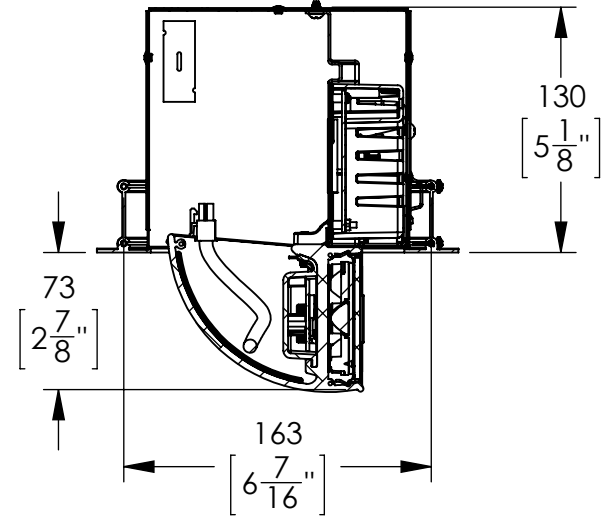
SECTION BF-BF SCALE 1 : 4
