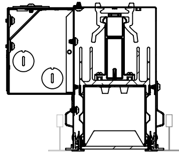
SECTION A-A STANDARD GRID
