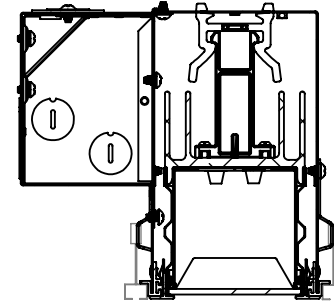
SECTION A-A SLOT-T GRID
