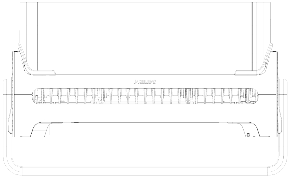
SPREAD LENS, FULL GLARE SHIELD
