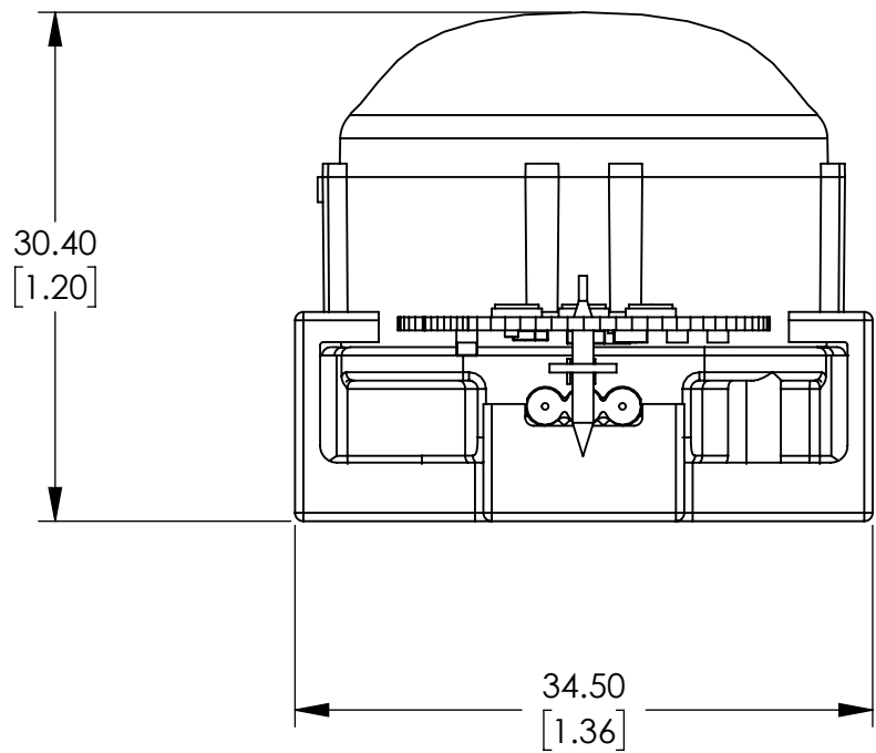
NARROW BEAM OPTIC LENS WITH SINGLE NODE MOUNT
