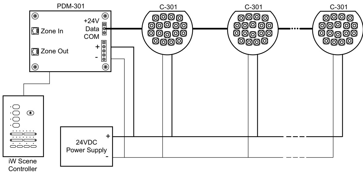
Typical installation using Color Kinetics PDM-301 Power/Data Module Multiple DLEs: 175ft max length from PDM to last DLE 1.5V max drop at last DLE under full load
