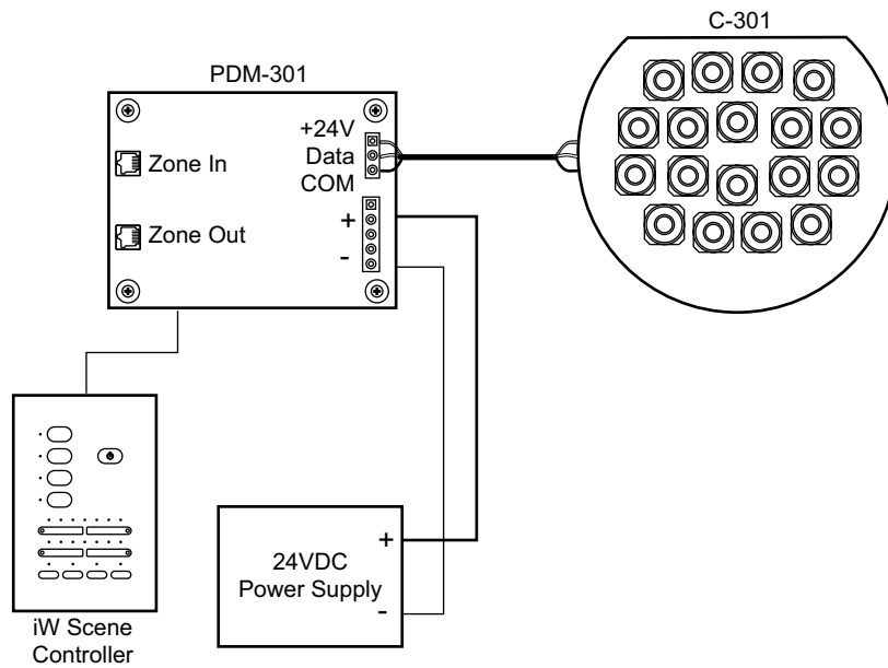
Typical Installation Using Color Kinetics PDM-301 Power/Data Module Single DLE: 25W Max Power Output
