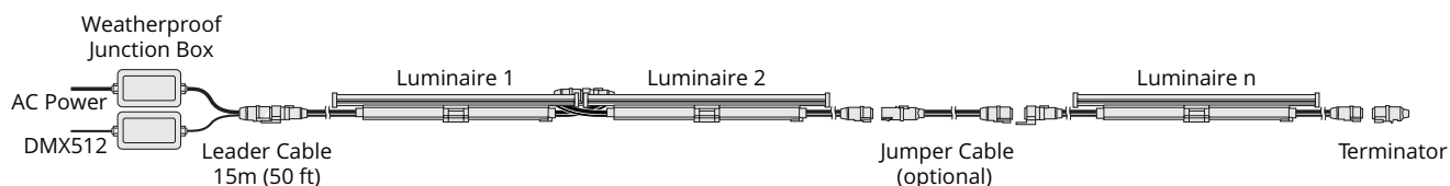
Jumper Cable (UL) 1.5 m (5ft)
